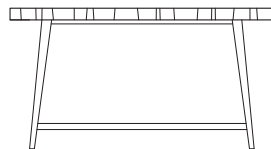
Sideboard VT40:135 h: 72 cm w: 45 cm l: 135 cm Top: Lacquered Stand: P2, P4 Top available in P4, please ask for price.
